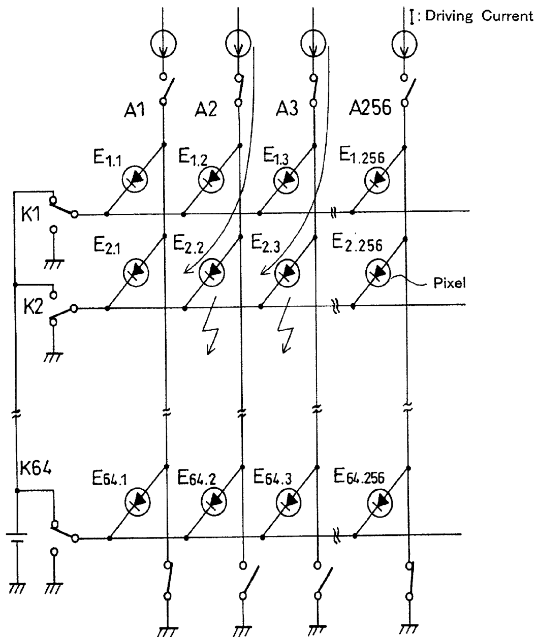
F I G . 2 5 (PRIOR ART)
